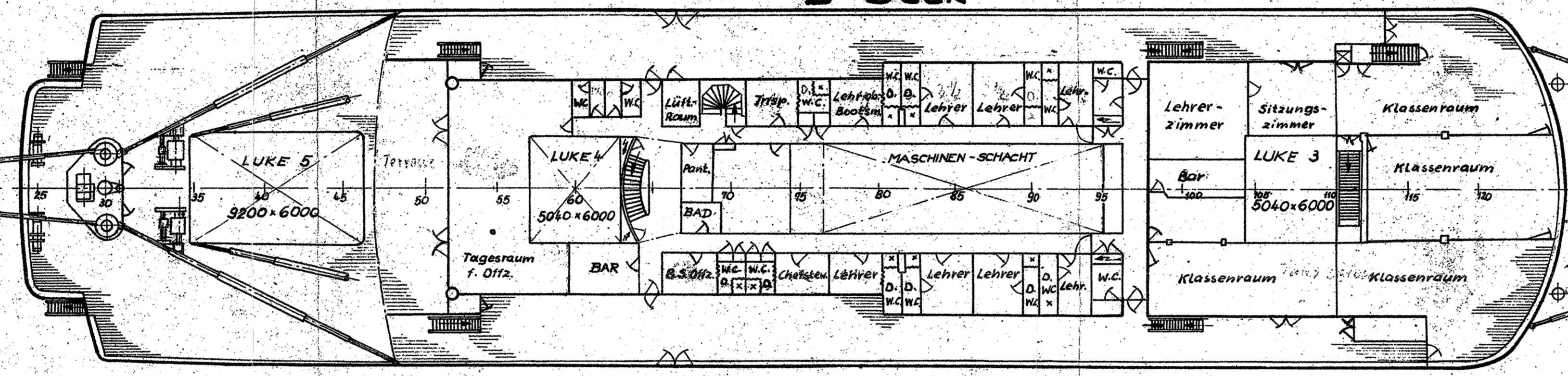
B-Deck
